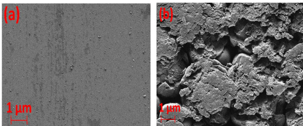
Scanning Electron Microscope (SEM) image of Europium nanoparticles with 50000x zoom
